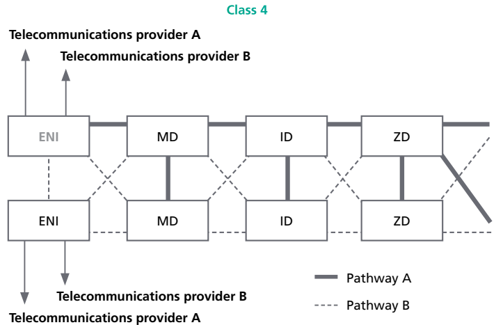
Figure 13: Fixed telecommunications cabling class 4 (Source: EN 50600-2-4)
