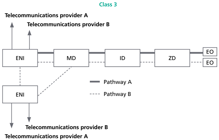
Figure 12: Fixed telecommunications cabling class 3 (Source: EN 50600-2-4)
