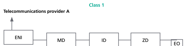
Figure 10: Telecommunications cabling class 1 using direct attached cords (Source: EN 50600-2-4)
