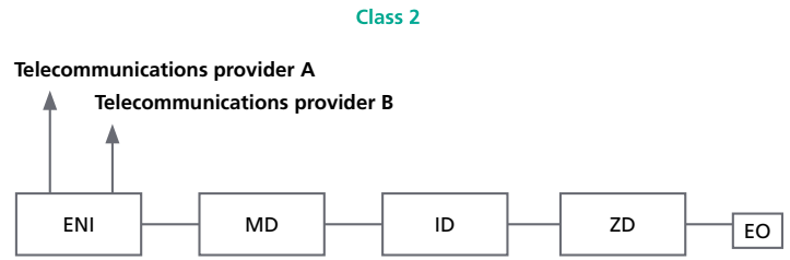
Figure 11: Fixed Telecommunications cabling class 2 (Source: EN 50600-2-4)
