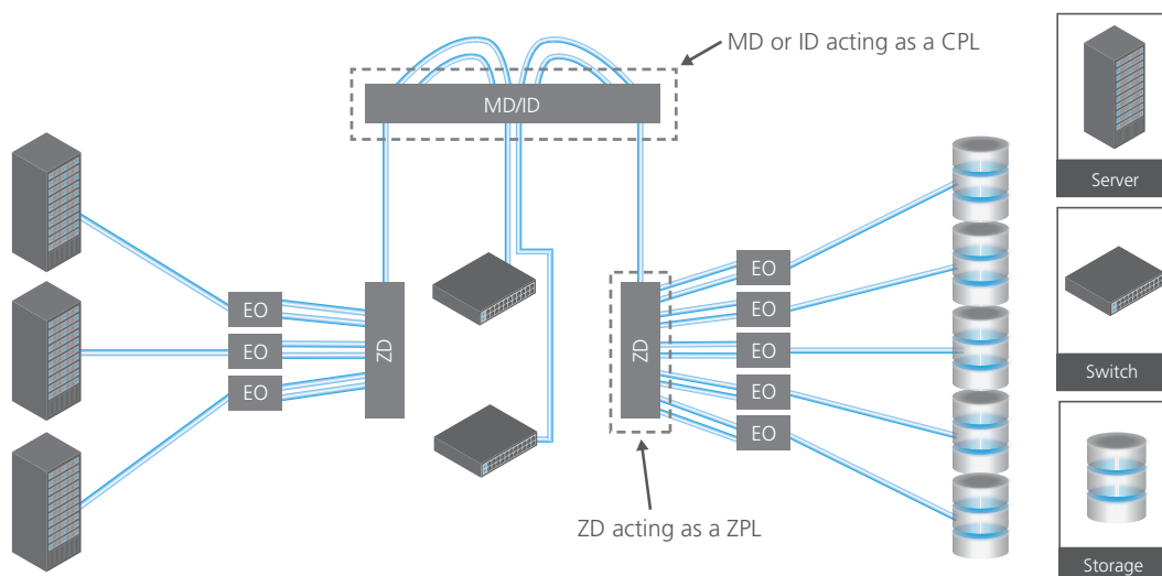
Figure 15: Moves, adds and changes using Cross-connects
