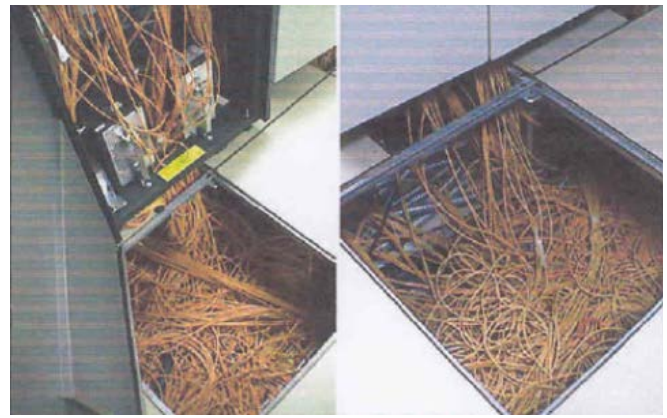
Figure 6: Example of unstructured growth of point-to-point cabling (Source: EN 50600-2-4)
