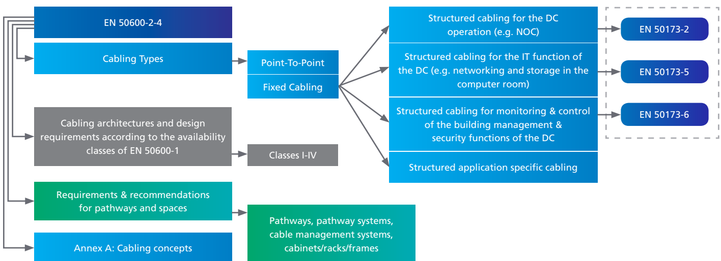
Figure 4: Content & structure of EN 50600-2-4
