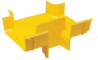
FiberGuide® Horizontal T with 4x6in Rear Downspout, 4x12in, Yellow
